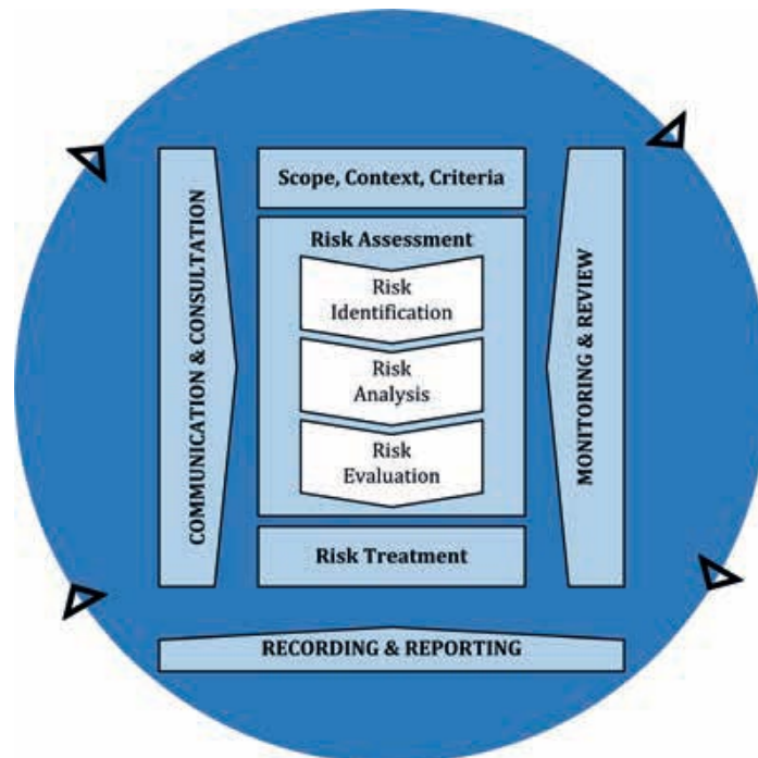
Figure 1: risk assessment 9
